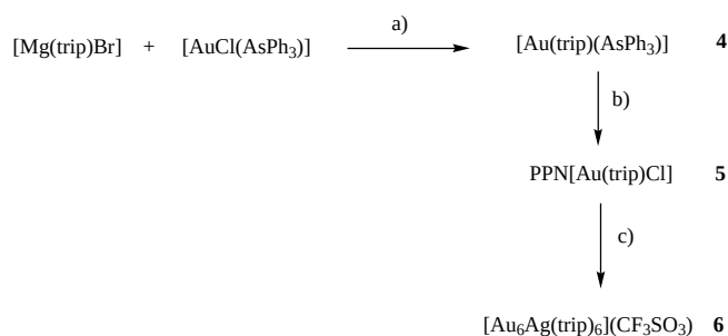
Scheme 2. Synthesis of complexes 4–6 . a) 0^\circ\text{C} (molar ratio 1.5:1); b) \text{PPN}^+\text{Cl}^- (molar ratio 1:1); c) [\text{Ag}(\text{CF}_3\text{SO}_3)] (molar ratio 1:1 or 1.25:1).
